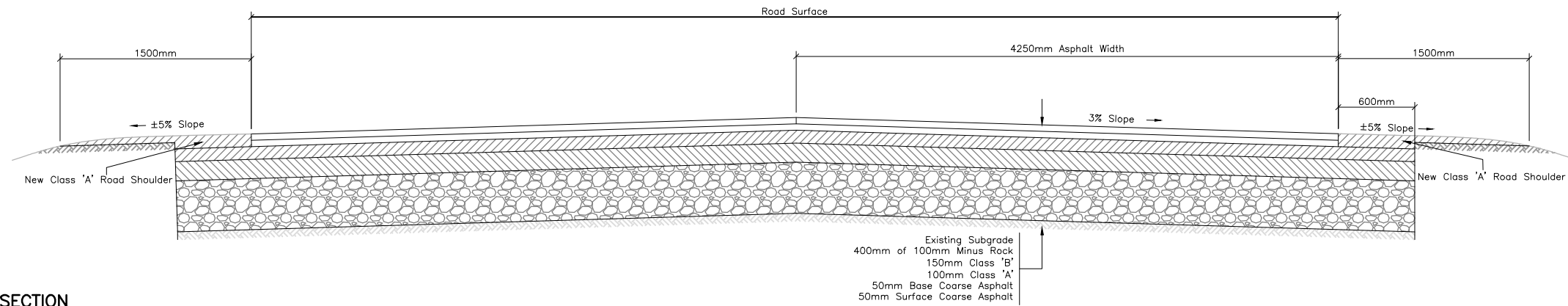
TYPICAL ROAD SECTION STA. 0+113.00 TO STA. 0+382.60
