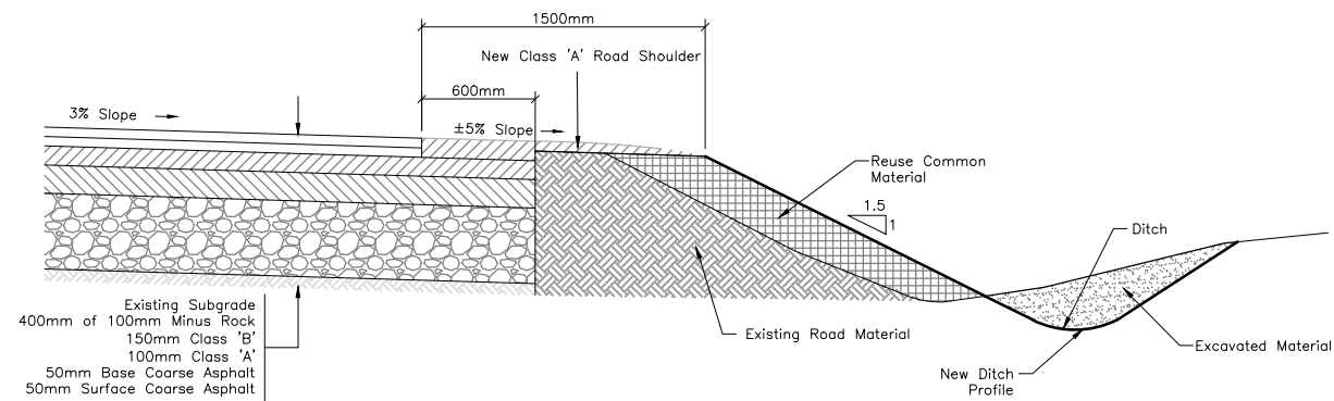
TYPICAL SECTION - ROADWAY WIDENING
