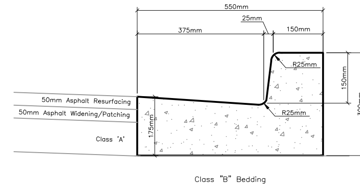
TYPICAL SECTION - CONCRETE CURB AND GUTTER
