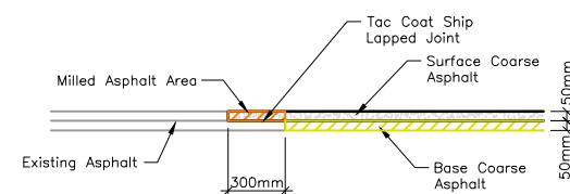
SHIPLAP JOINT - NEW ASPHALT TO EXISTING ASPHALT
