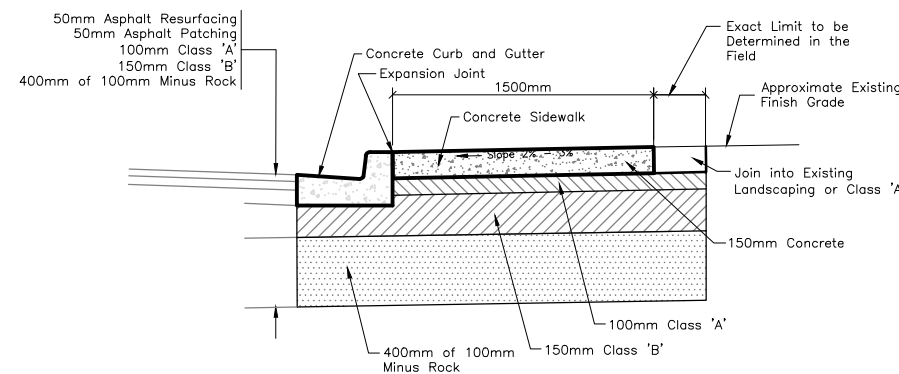
TYPICAL SECTION - CONCRETE CURB/GUTTER AND SIDEWALK
