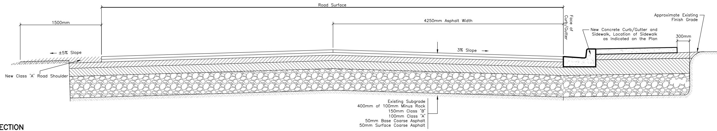
TYPICAL ROAD SECTION STA. 0+068.50 TO STA. 0+113.00
