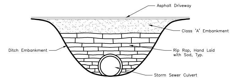
TYPICAL STORM CULVERT RIP RAP DETAIL
